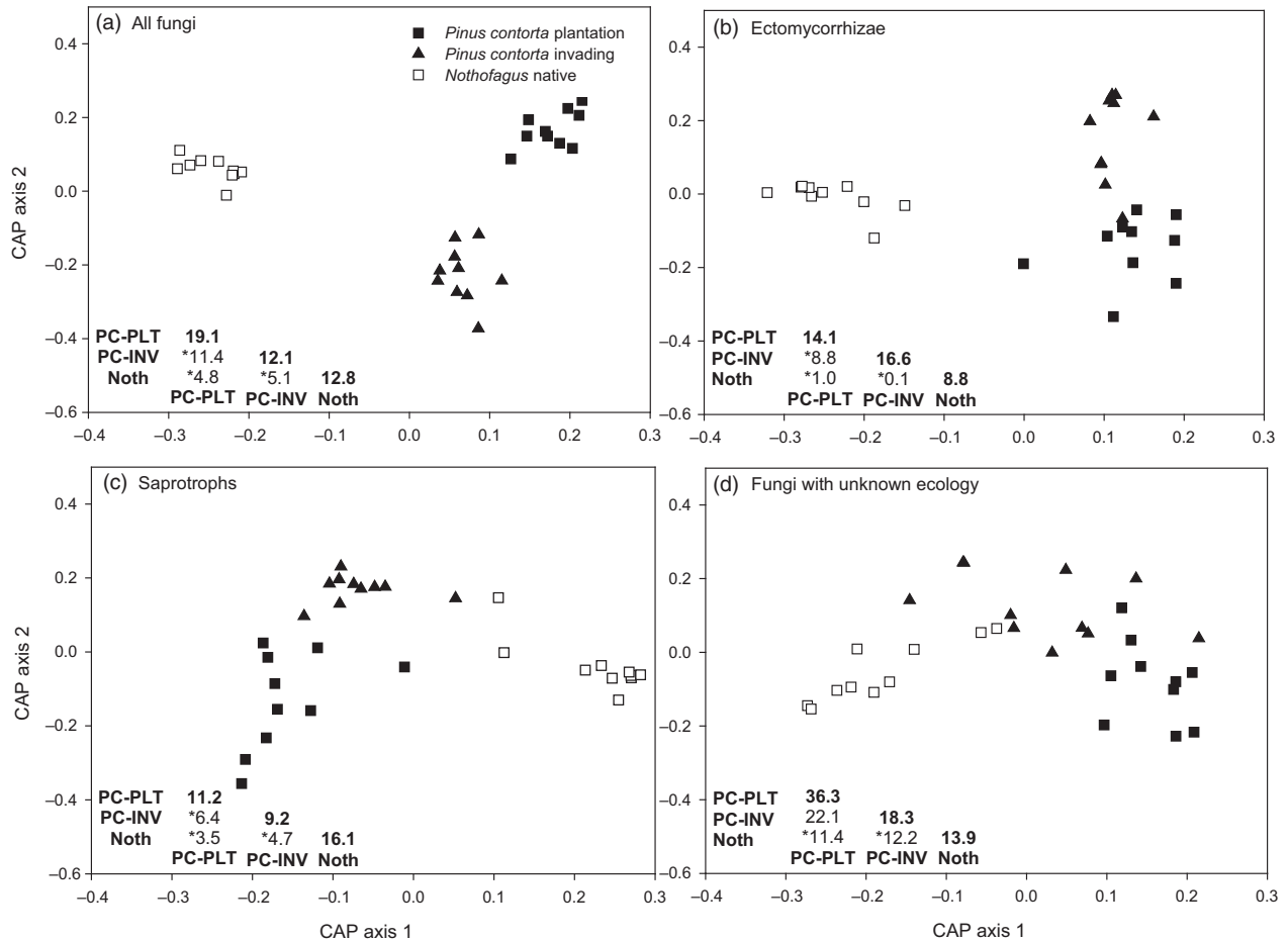
Fig. 6. A constrained ordination (canonical analysis of principal coordinates; CAP) showing the results of a PERMANOVA (permutational multivariate analysis of variance) test evaluating the community composition of (a) total fungal root endophytes, (b) ectomycorrhizal fungi, (c) saprotrophic fungi and (d) fungi with unknown ecology associated within the roots of three Southern Hemisphere tree types, source Pinus contorta plantations (PC-PLT), invading P. contorta individuals (PC-I) and native Nothofagus trees (Noth). In the lower left corner of each panel, the similarity (%) of fungal communities among sites within each group is listed in bold, whereas pairwise similarities between groups are non-bolded. An asterisk next to pairwise similarity values indicate when post hoc pairwise PERMANOVA analyses indicated a significant differences (at P < 0.05 ) in community composition. *For community composition data, the F-value is generated using permutations procedures and thus is referred to as a Pseudo- F-value.
