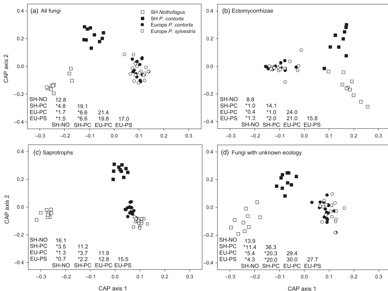
Fig. 4. A constrained ordination (canonical analysis of principal coordinates; CAP) showing the results of a PERMANOVA (permutational multivariate analysis of variance) test evaluating the effect of tree type (introduced Pinus contorta (PC) vs. the most similar dominant native tree species) and region (Europe = EU, or Southern Hemisphere = SH) on community composition of (a) total root fungal endophytes (b) ectomycorrhizal fungi, (c) saprotrophic fungi or (d) fungi with unknown ecology. The native trees in the Southern Hemisphere locations were Nothofagus sp. (NO) and Pinus sylvestris (PS) in European locations. In the lower left corner of the figure, similarity (%) of fungal communities across sites within each group is listed in bold, while pairwise similarities between groups are non-bolded. An asterisk next to pairwise similarity values indicates when post hoc pairwise PERMANOVA analyses indicated a significant difference ( P < 0.05 ) in community composition. *For community composition data, the F-value is generated using permutations procedures and thus is referred to as a Pseudo- F-value.
