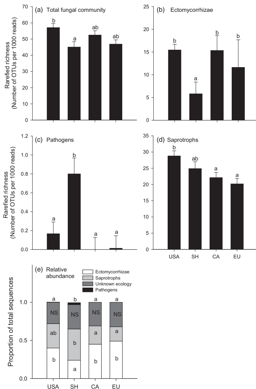
Fig. 3. Operational taxonomic unit (OTU) richness (a-d) and relative abundance (e) of fungal endophyte communities associated with Pinus contorta roots in two native range source populations (USA and Canada (CA)) and two sink populations (Southern Hemisphere (SH) or Europe (EU)), respectively. Richness is presented as the average rarefied richness (for 1000 sequence reads) for each sample. Results from corresponding two-way ANOVA are reported for all variables are reported in Table 1, except for pathogens which were compared using a Kruskal–Wallis test. Different letters above bars or across bar segments (a or b) with the same shade indicate significant pairwise differences determined using Tukey's post hoc tests, except for pathogens (e) which were compared using nonparametric post hoc comparisons.
