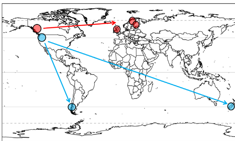
Fig. 1. A map of two Pinus contorta source–sink pairs (SSP). The northern SSP is depicted in red, with native range locations occurring in northern British Columbia, Canada and corresponding introduced populations in Scotland, Sweden and Finland. The southern SSP is depicted in blue, with native range populations occurring the Pacific Northwest, USA, and corresponding introduced populations in Chile and New Zealand.
