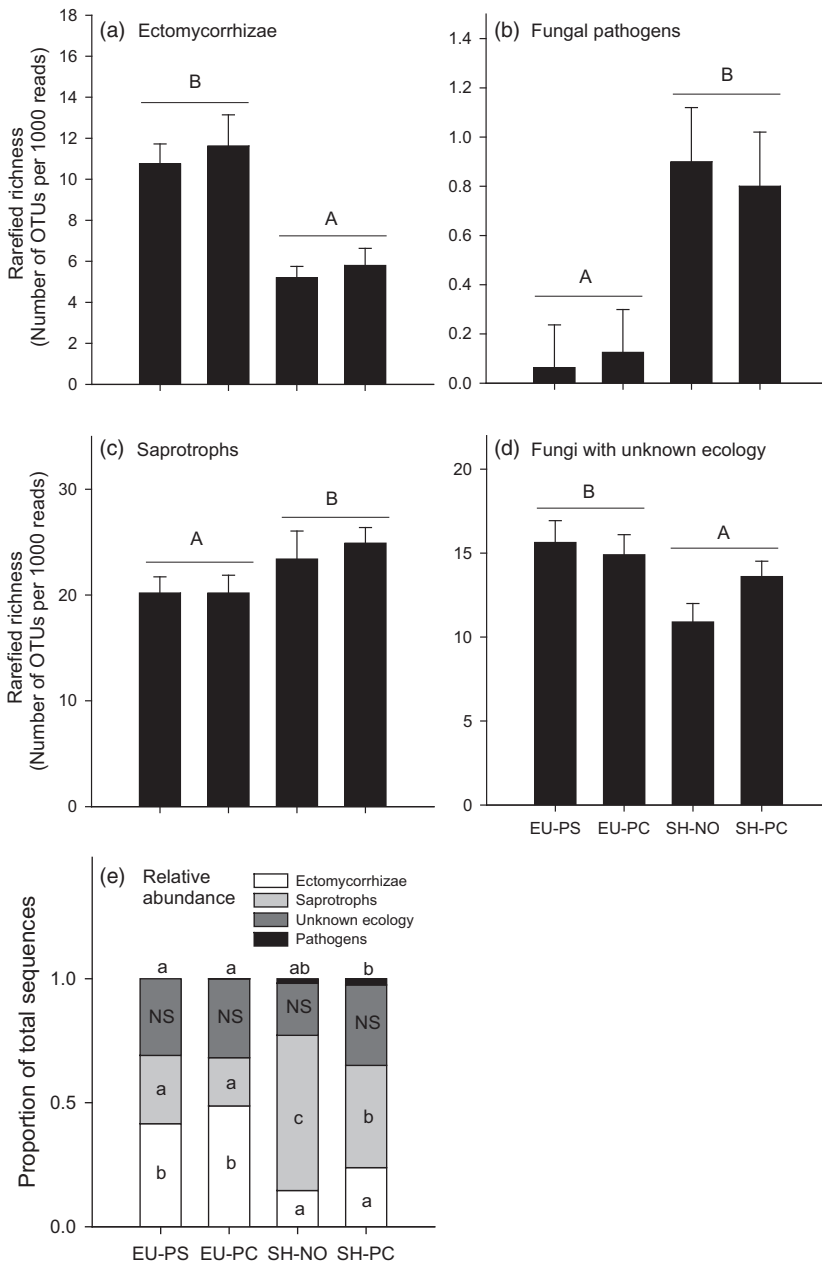
Fig. 5. Differences in operational taxonomic unit (OTU) richness (a-d) and relative abundance (e) of fungal root endophyte communities associated with either Pinus contorta (PC) or Pinus sylvestris (PS) in Europe (EU), or P. contorta or Nothofagus sp. (NO) in the Southern Hemisphere (SH). Richness is presented as the average rarefied richness (for 1000 sequence reads) for each sample. Results from a corresponding two-way ANOVA are reported in Table 2. Different letters above bars or across bar segments (a or b) with the same shade indicate significant pairwise differences determined using Tukey's post hoc tests, except for pathogens (e) which were compared using nonparametric post hoc comparisons.
