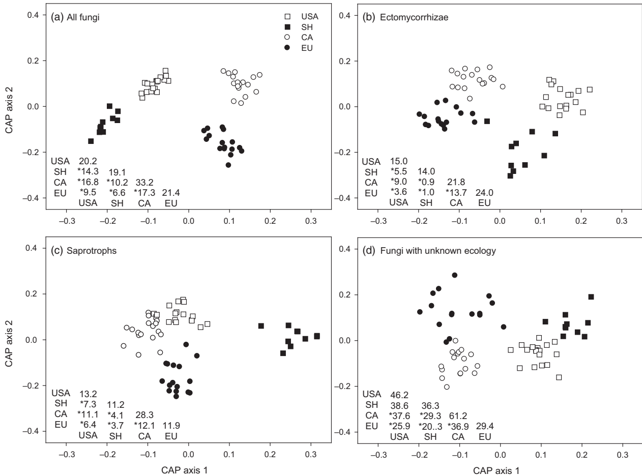
Fig. 2. A constrained ordination (canonical analysis of principal coordinates; CAP) showing the results of a PERMANOVA (permutations multivariate analysis of variance) test evaluating differences in community composition of (a) total fungal endophytes, (b) ectomycorrhizas, (c) saprotrophic fungi and (d) fungi with unknown ecology associated with Pinus contorta roots growing in four distinct regions (United States of America = USA, Canada = CA, Southern Hemisphere = SH, and Europe = EU). Results of the PERMANOVA are reported in Table 1. In the lower left corner of each panel, within group similarity (%) are listed in bold, while pairwise similarities between groups are non-bold. An asterisk next to pairwise similarity values indicate when post hoc pairwise PERMANOVA analyses indicated a significant difference ( P < 0.05 ) in community composition between the two regions. *For community composition data, the F-value is generated using permutations procedures and thus is referred to as a Pseudo- F-value.
