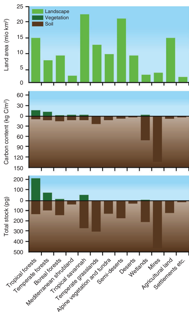
FIGURE 1 | Area, stored carbon (in kg/m 2 ) and total global above and below ground carbon (Petagram, Pg) of the most important biomes worldwide. Modified from Ref 19.
